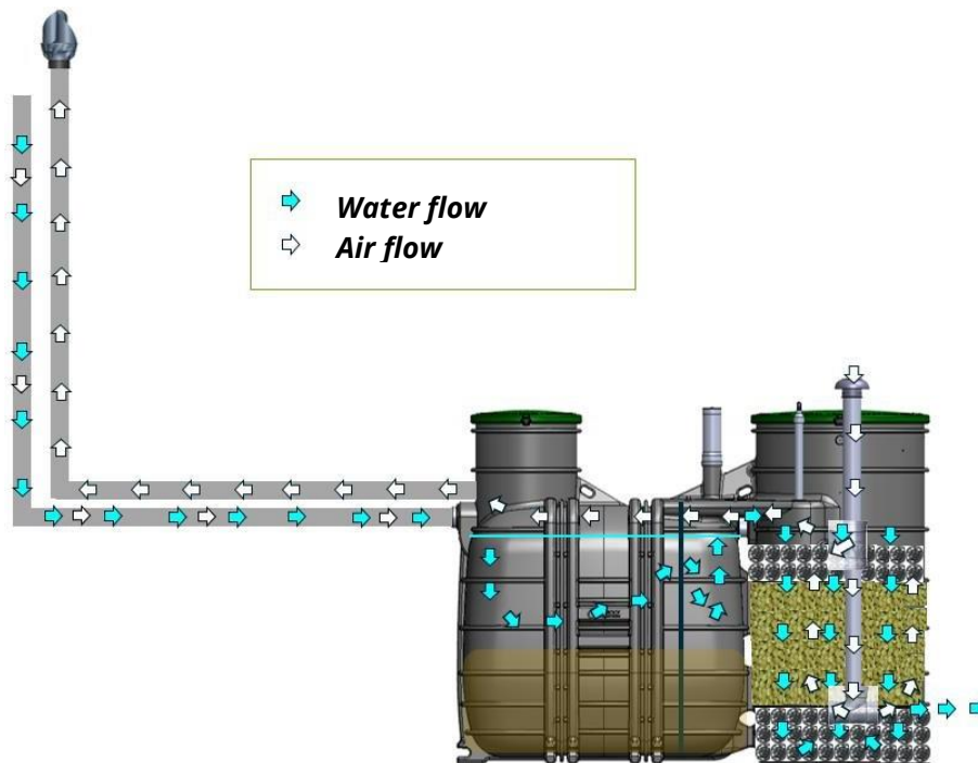
Diagram of the water circulation and ventilation
