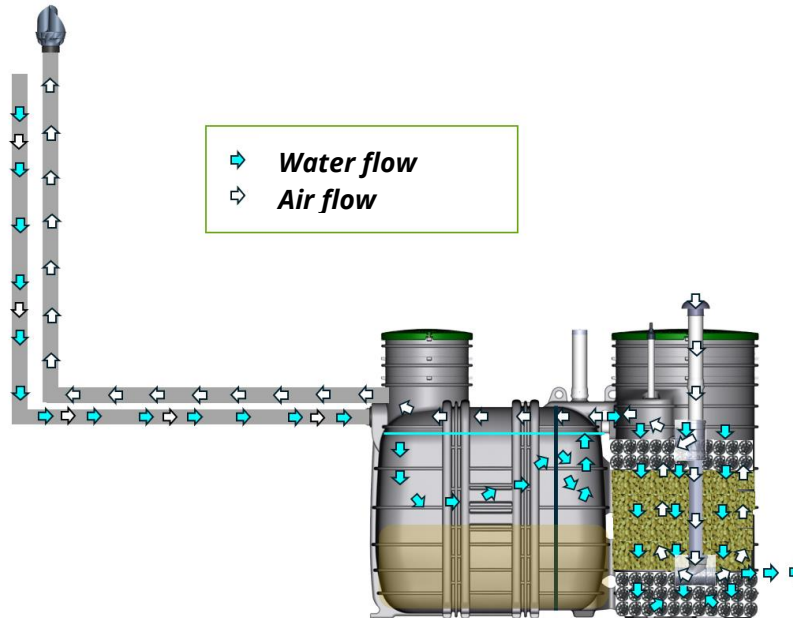
Diagram of the water circulation and ventilation
